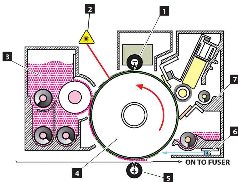
Electrophotographic Imaging System
